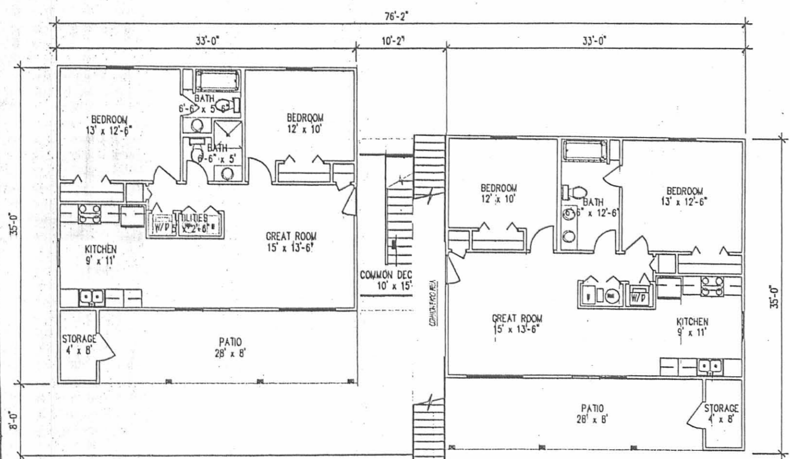
QUAD FIRST FLOOR PLAN (right)
