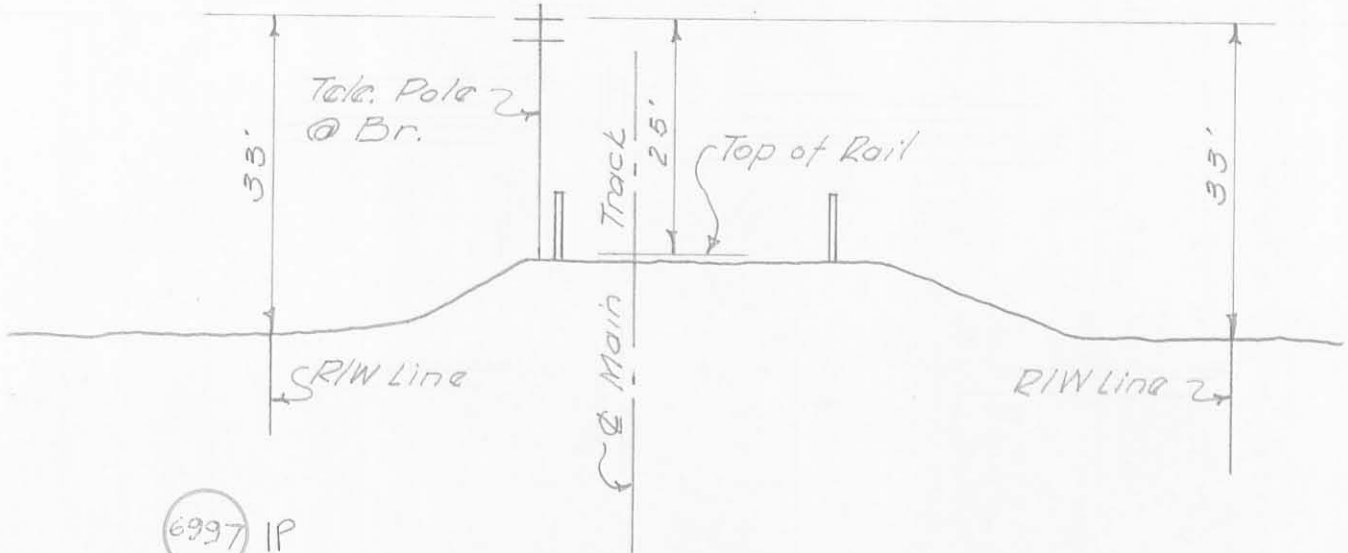
PROFILE AT CROSSING 1" = 20'
