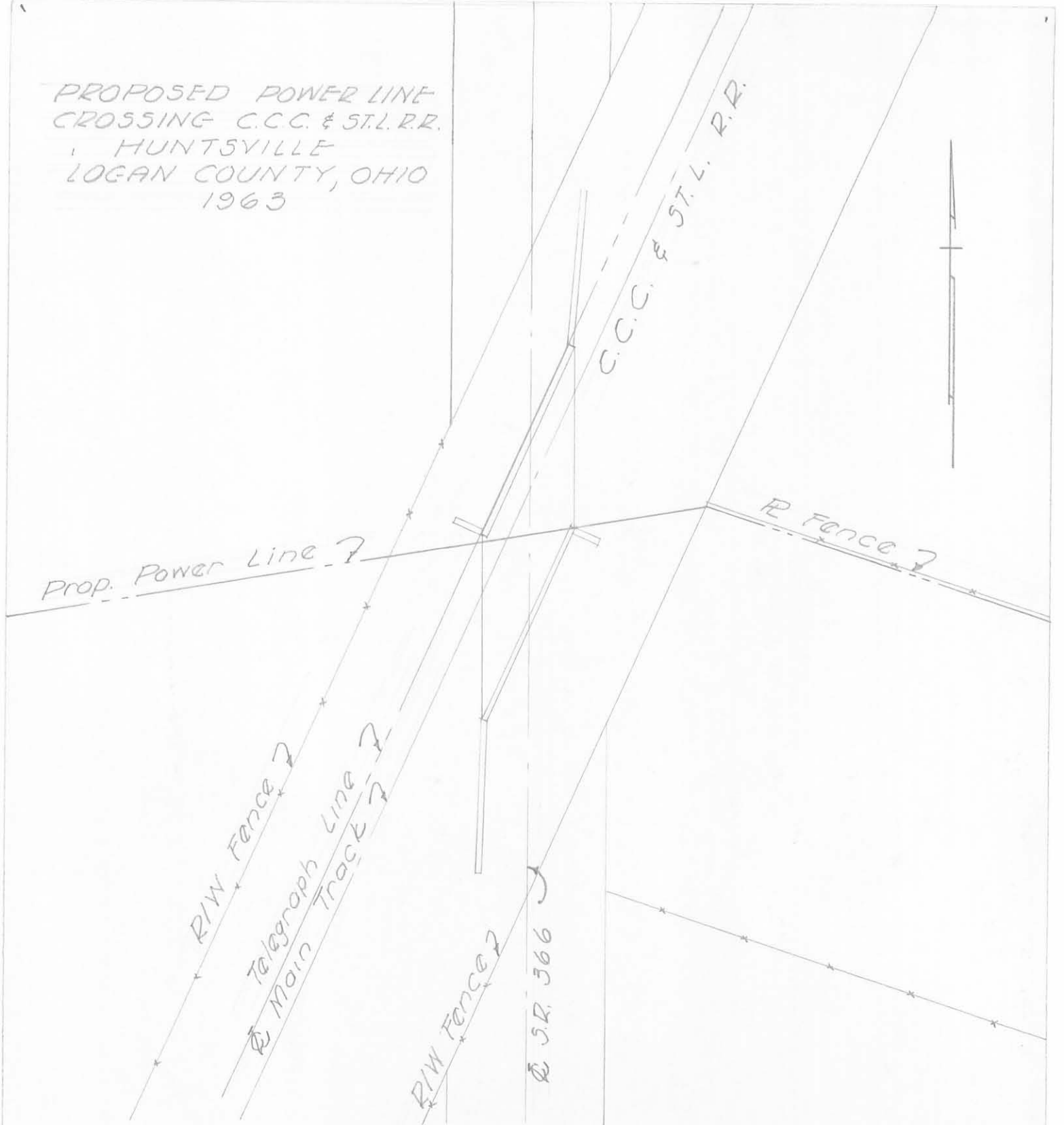
SITE PLAN 1" = 50'
